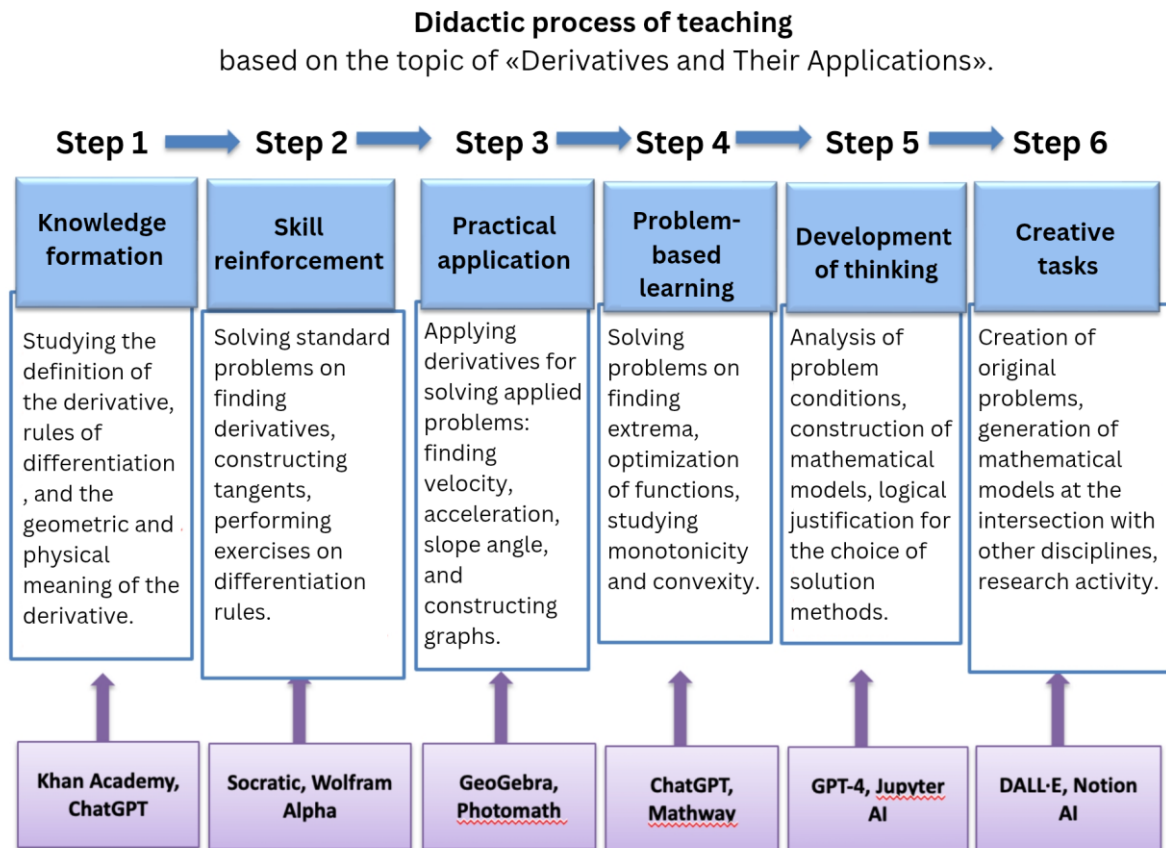
Fig. 3. Didactic process of teaching, using the example of the topic "Derivatives and Their Applications."
